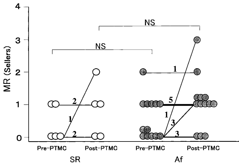
Fig. 1 Angiographic changes observed in mitral regurgitation before (Pre) and after (Post) PTMC in the two groups. MR = mitral regurgitation. Other abbreviations as in Table 1.
