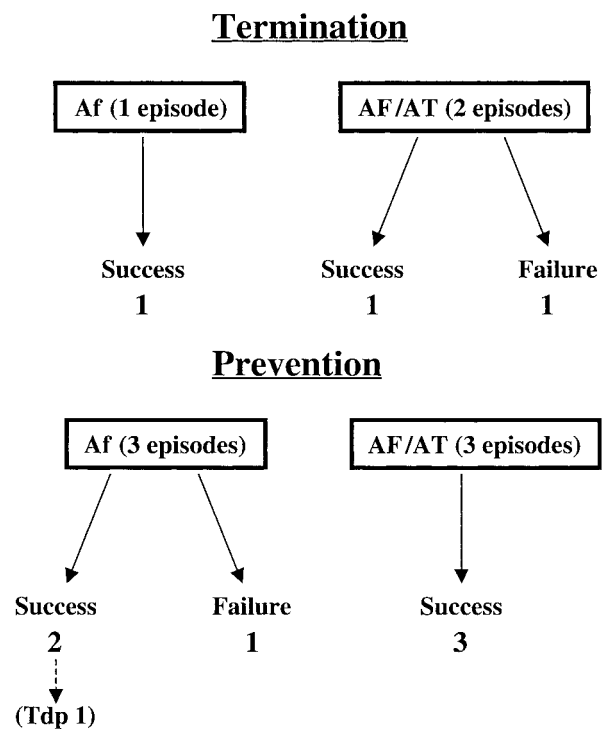
Fig. 2 Efficacy of nifekalant for the termination or prevention of atrial tachyarrhythmia in patients with severe heart failure Tdp=torsades de pointes. Other abbreviations as in Table 1.
