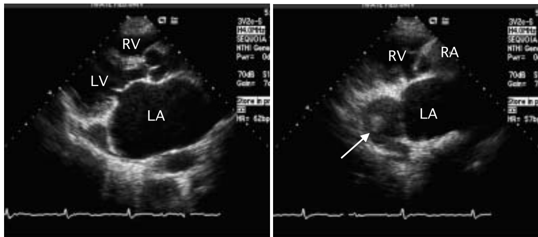
Fig. 3 Transthoracic echocardiograms
